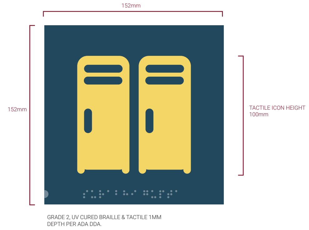
FRONT VIEW Scale 1:2
